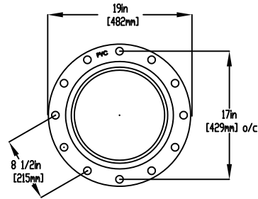
FLANGE DETAILS
