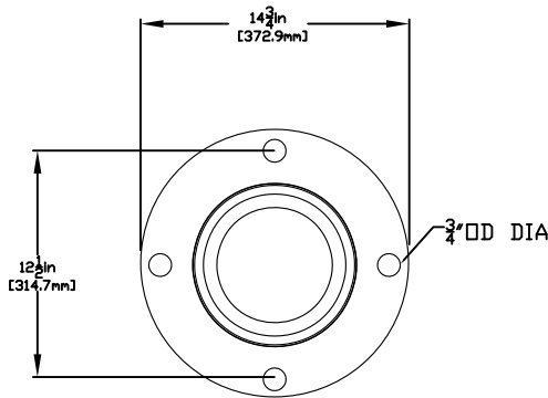
FLANGE DETAIL
