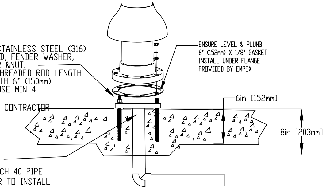
FLANGE DETAIL
