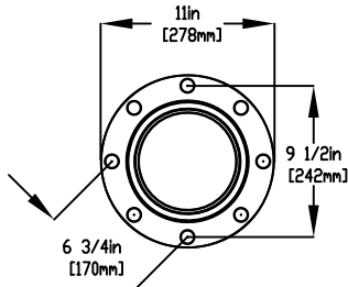
FLANGE DETAIL
