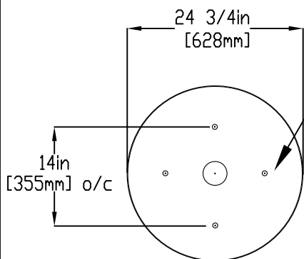
MOUNTING PLATE DETAIL
