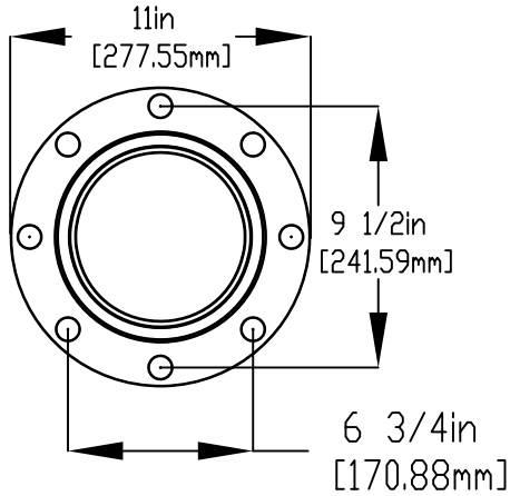
FLANGE DETAIL
