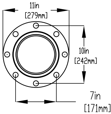
FLANGE DETAIL
