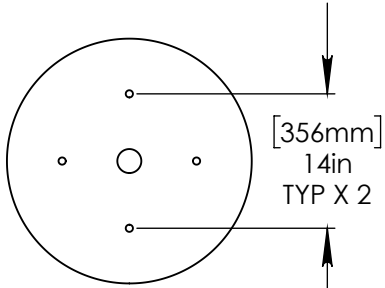
FLANGE DETAIL
