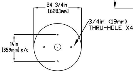
MOUNTING PLATE DETAIL
