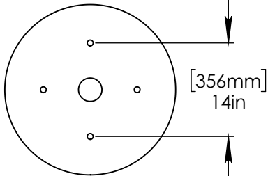
FLANGE DETAIL
