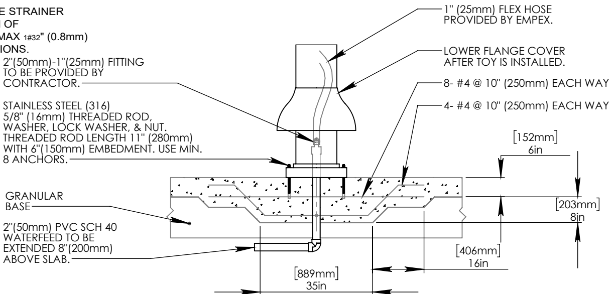
FLANGE DETAIL
