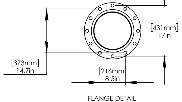
FLANGE DETAIL
