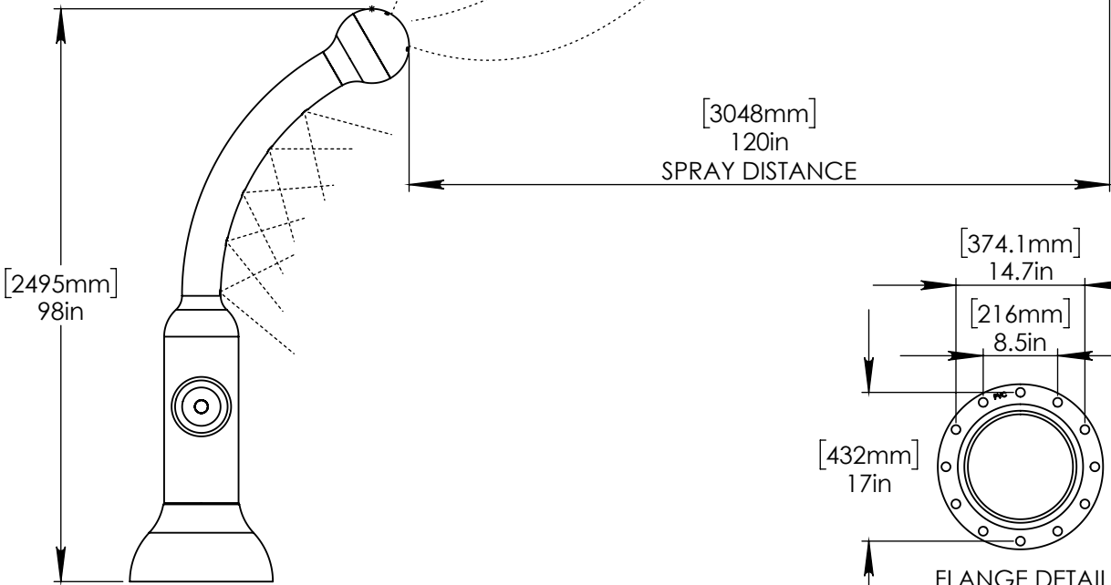
FLANGE DETAIL
