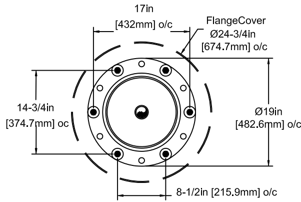
FLANGE DETAIL
