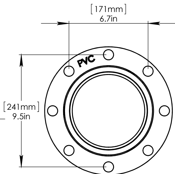
FLANGE DETAIL
