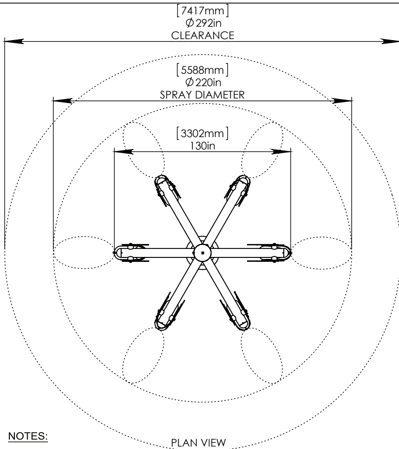
PLAN VIEW
