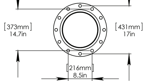
FLANGE DETAIL
