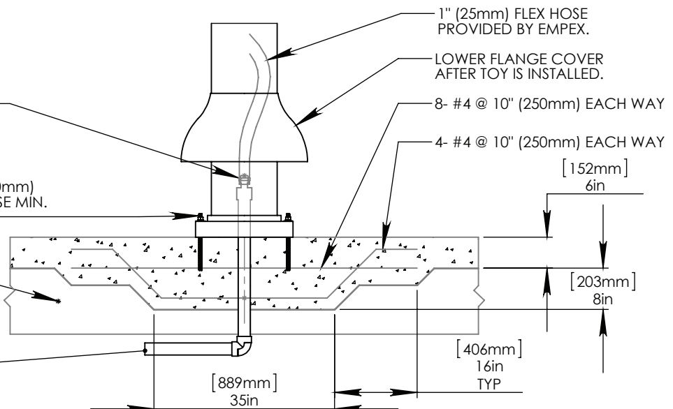
FLANGE DETAIL
