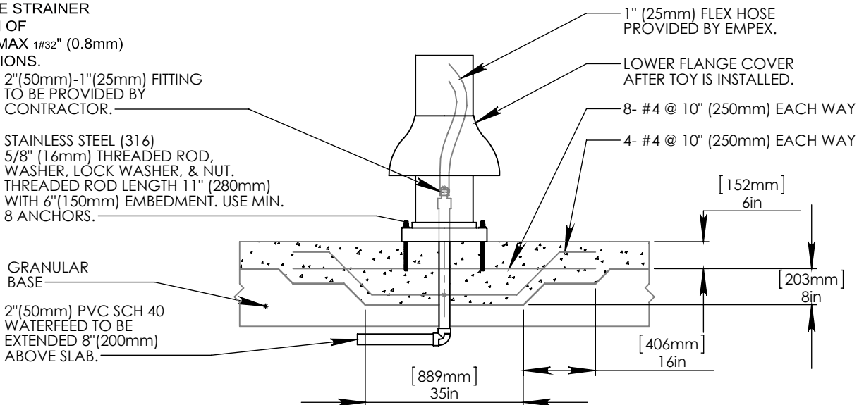
FLANGE DETAIL
