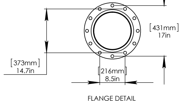
FLANGE DETAIL
