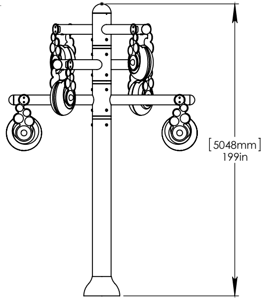
ELEVATION VIEW
