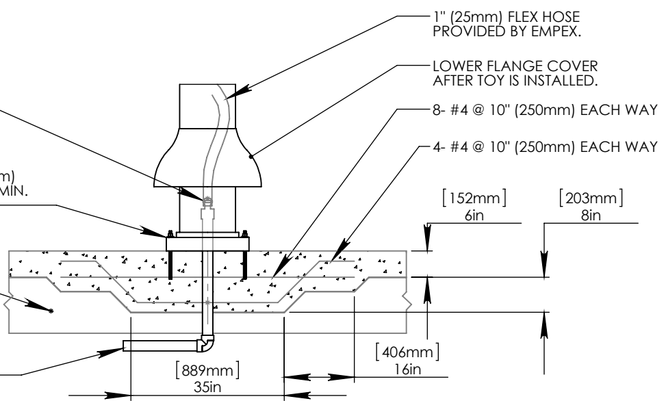
FLANGE DETAIL
