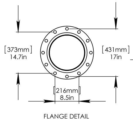
FLANGE DETAIL
