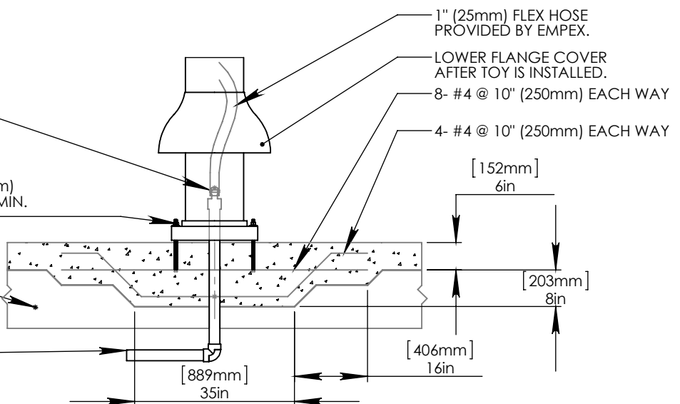
FLANGE DETAIL
