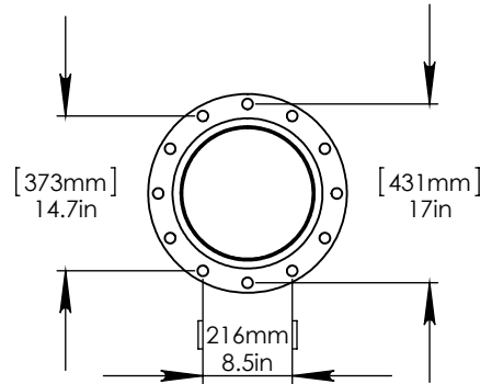
FLANGE DETAIL
