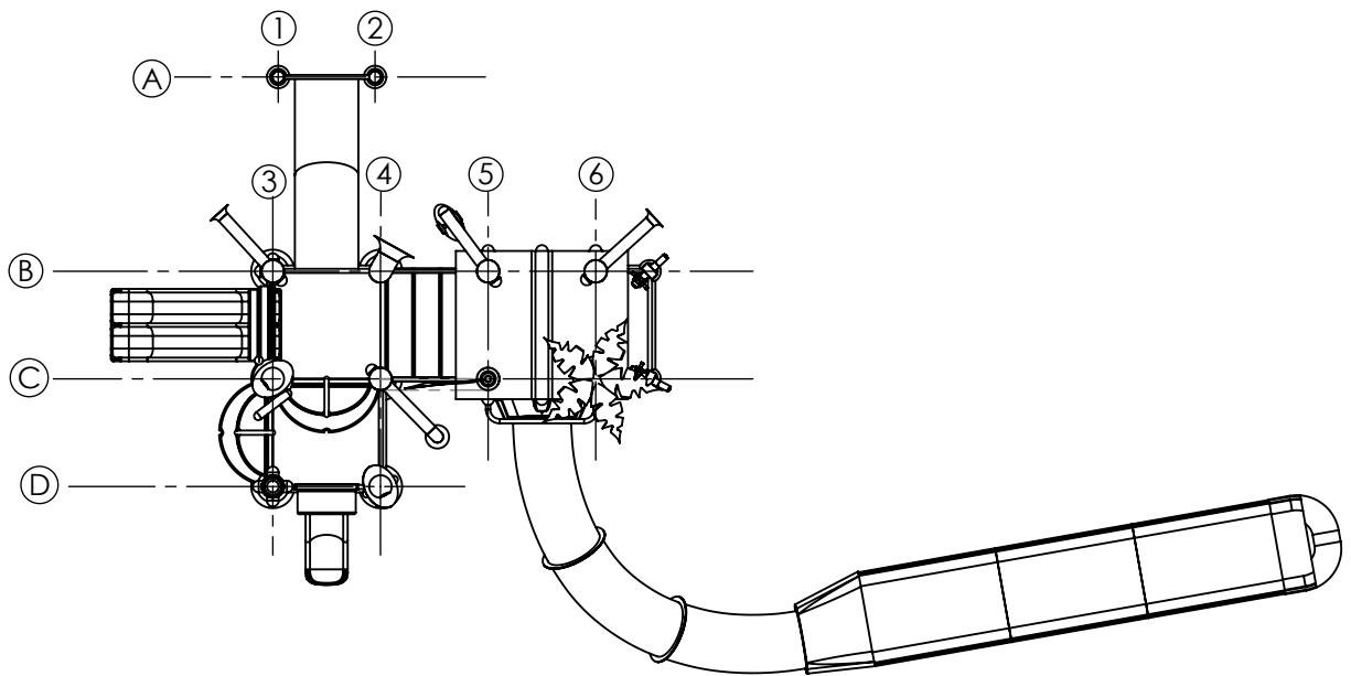
12" AQUADEK COLUMN MOUNTING FLANGE DETAIL.
