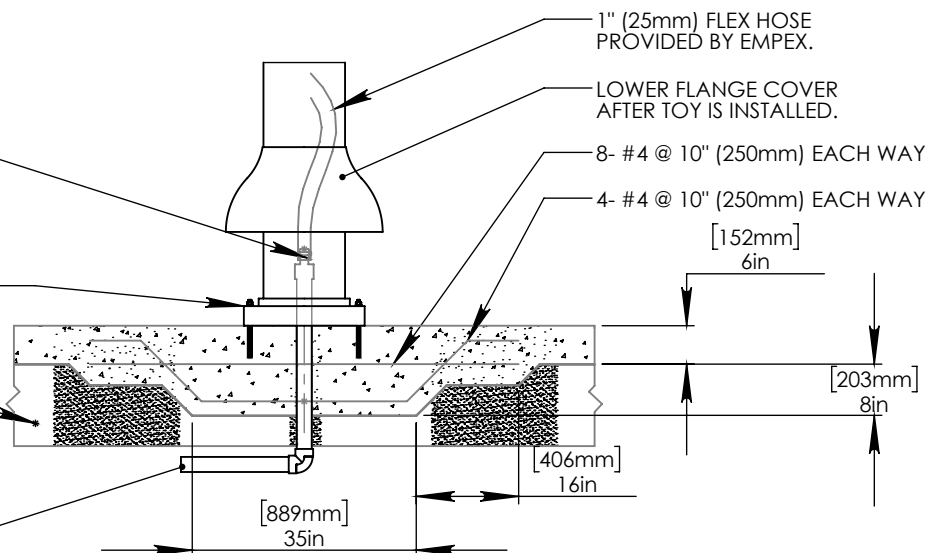
FLANGE DETAIL
