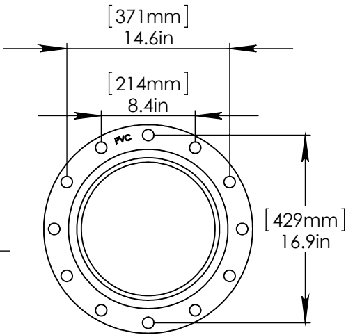
FLANGE DETAIL
