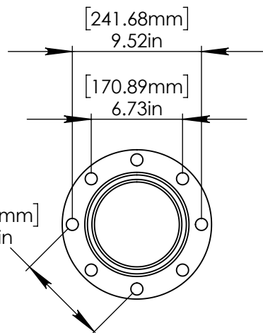
FLANGE DETAIL
