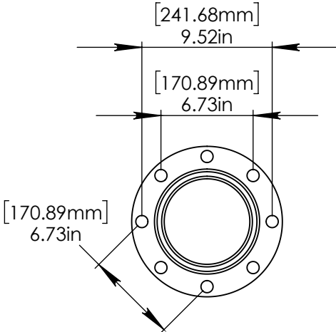
FLANGE DETAIL
