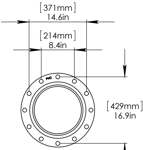
FLANGE DETAIL
