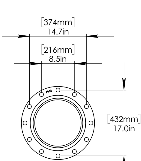
FLANGE DETAIL
