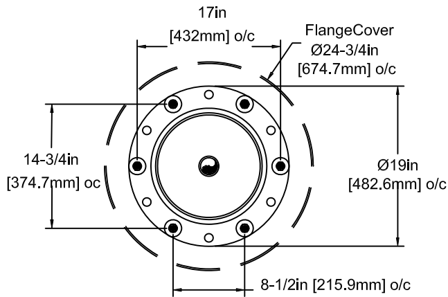
FLANGE DETAIL
