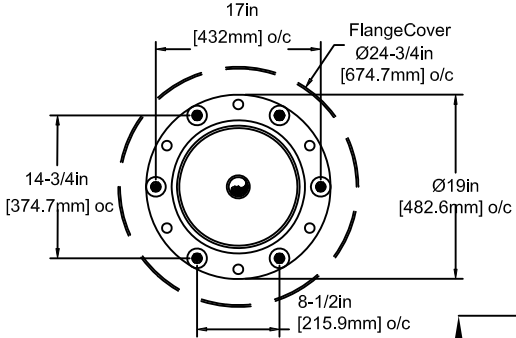
FLANGE DETAIL
