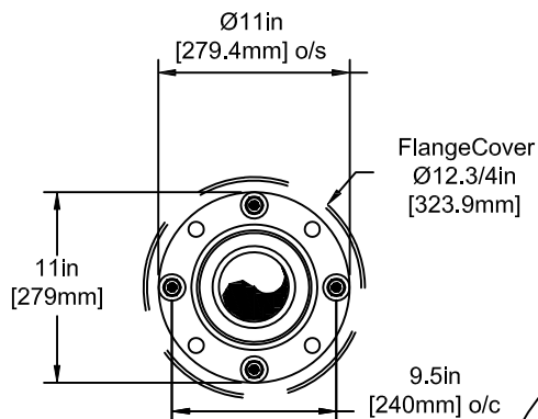
FLANGE DETAIL
