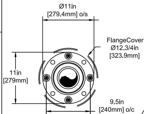
FLANGE DETAIL
