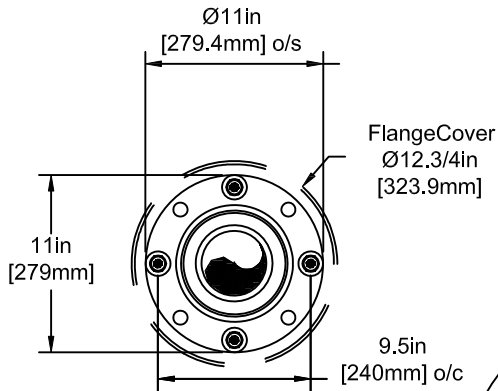
FLANGE DETAIL
