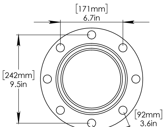
FLANGE DETAIL
