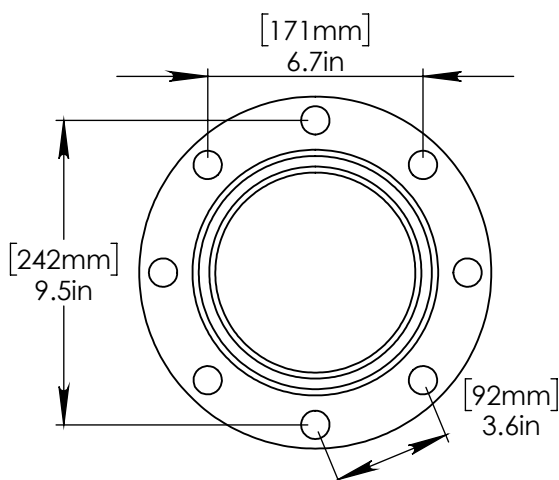
FLANGE DETAIL
