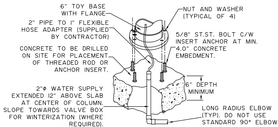
3 INSTALLATION DETAIL
