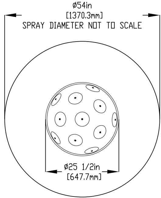
PLAN VIEW
