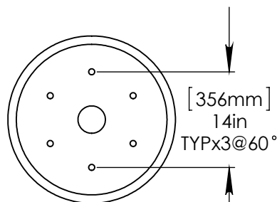
BOTTOM VIEW ANCHOR PATTERN
