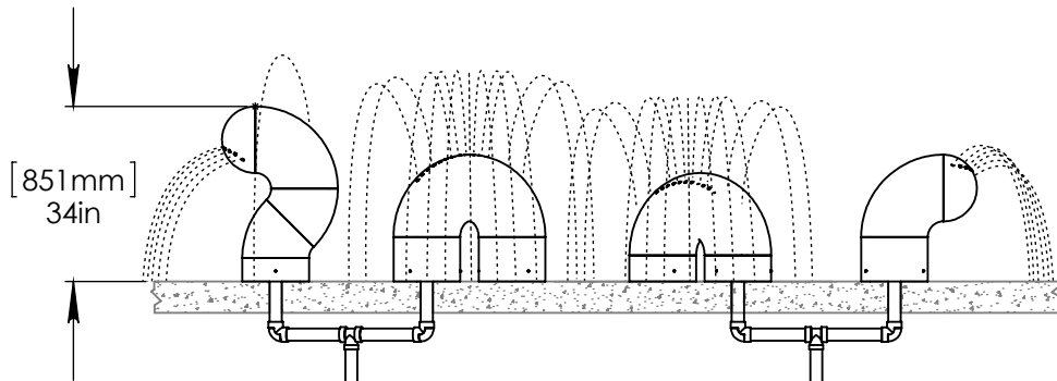
ELEVATION VIEW
