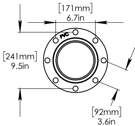
FLANGE DETAIL
