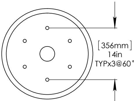
FLANGE DETAIL
