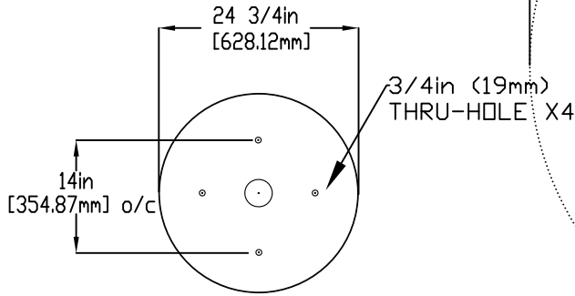
MOUNTING PLATE DETAIL
