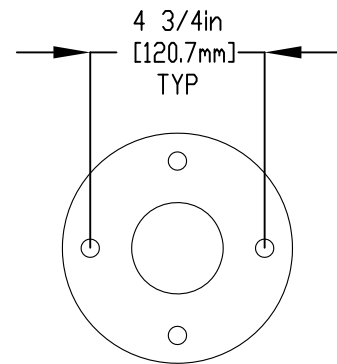
FLANGE DETAIL
