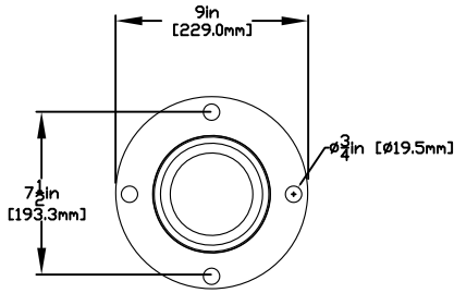
FLANGE DETAIL
