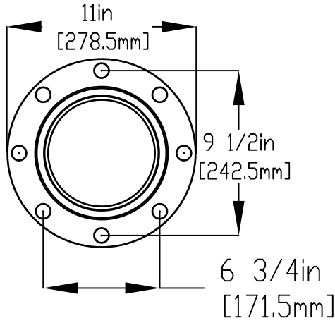
FLANGE DETAIL
