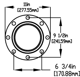
FLANGE DETAIL
