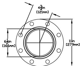
FLANGE DETAIL
